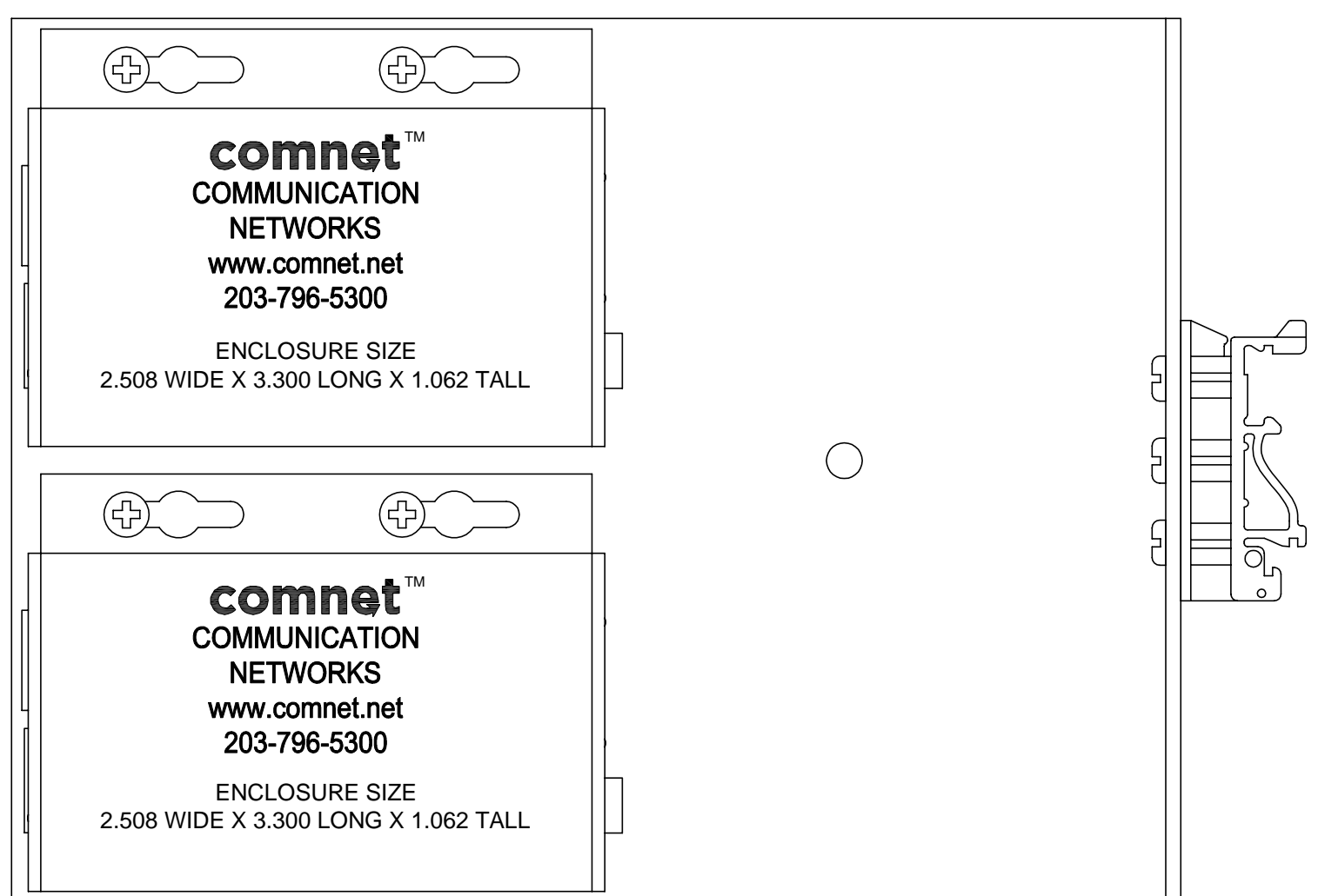
ENCLOSURES IN HORIZONTAL POSITION USE HOLES CODED "A", "B", "J" AND "K"
