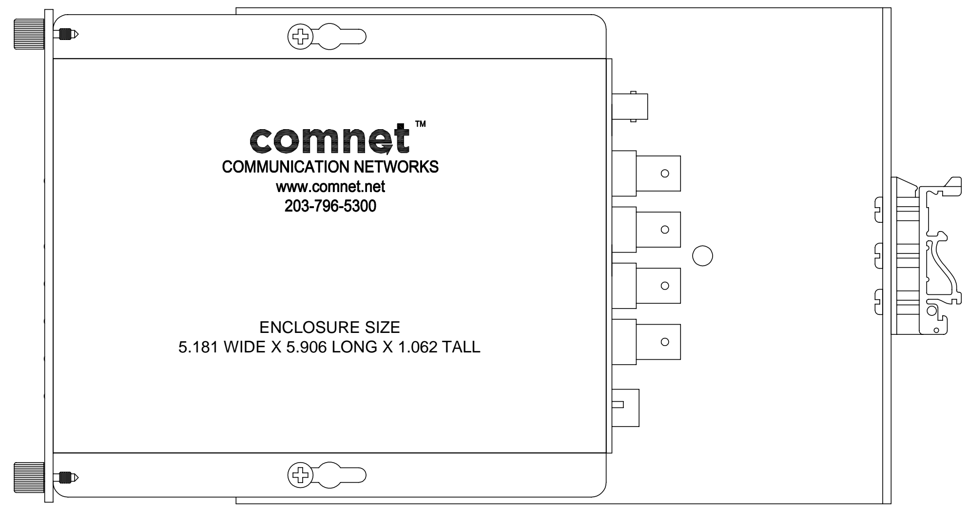
ENCLOSURE MOVED FOWARD FOR CABLE ACCESS IN THE REAR USE HOLES CODED "A" AND "P"
