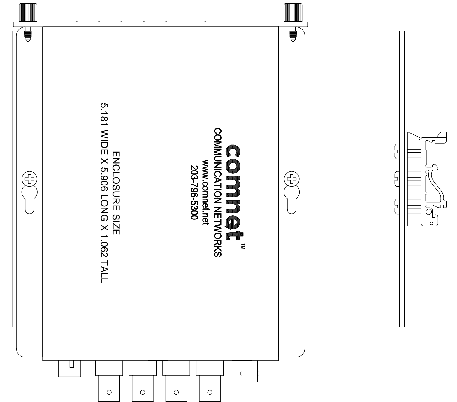
ENCLOSURE IN VERTICAL POSITION USE HOLES CODED "F" AND "H"
