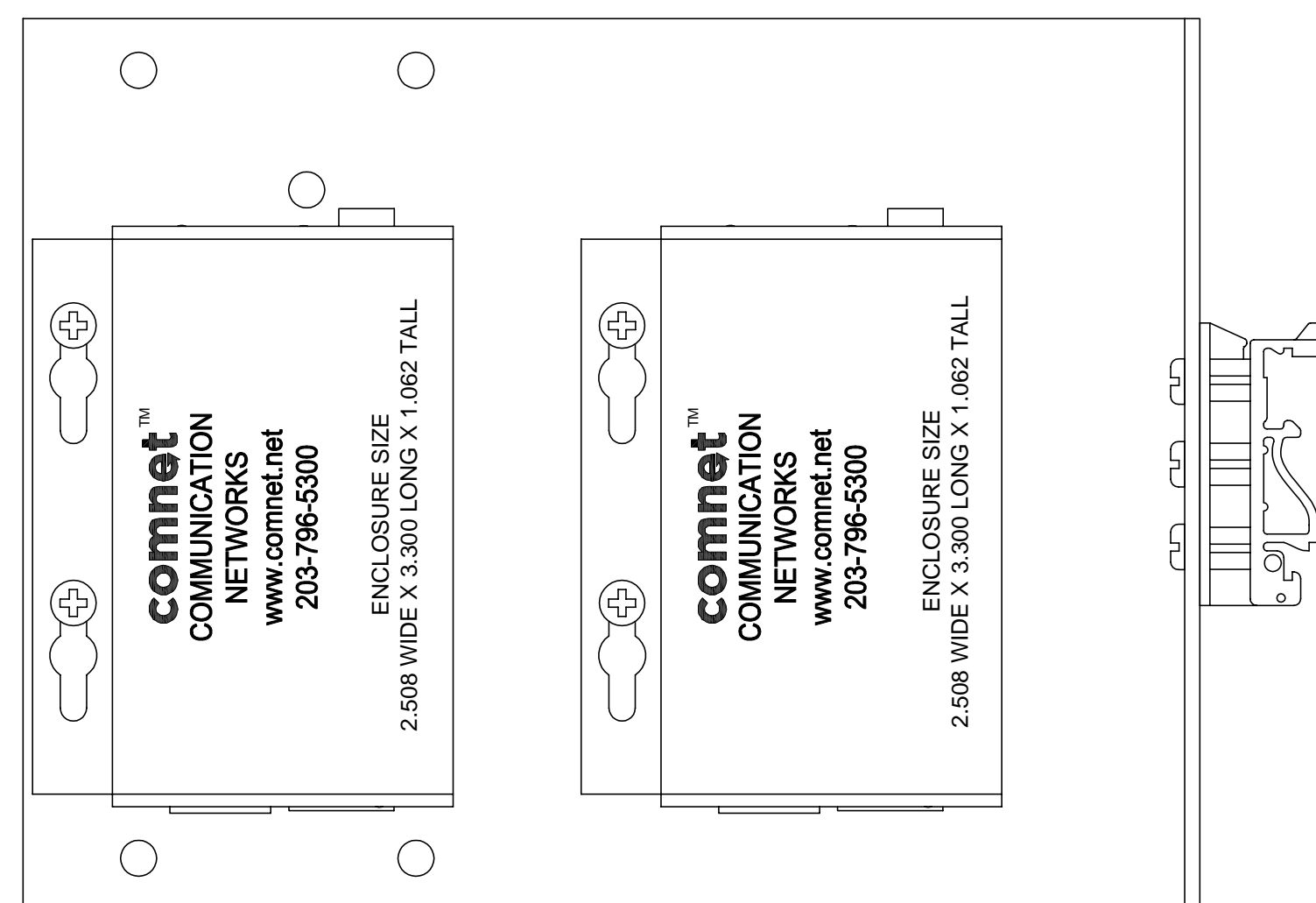
ENCLOSURES IN VERTICAL POSITION USE HOLES CODED "D", "E", "L" AND "M"
