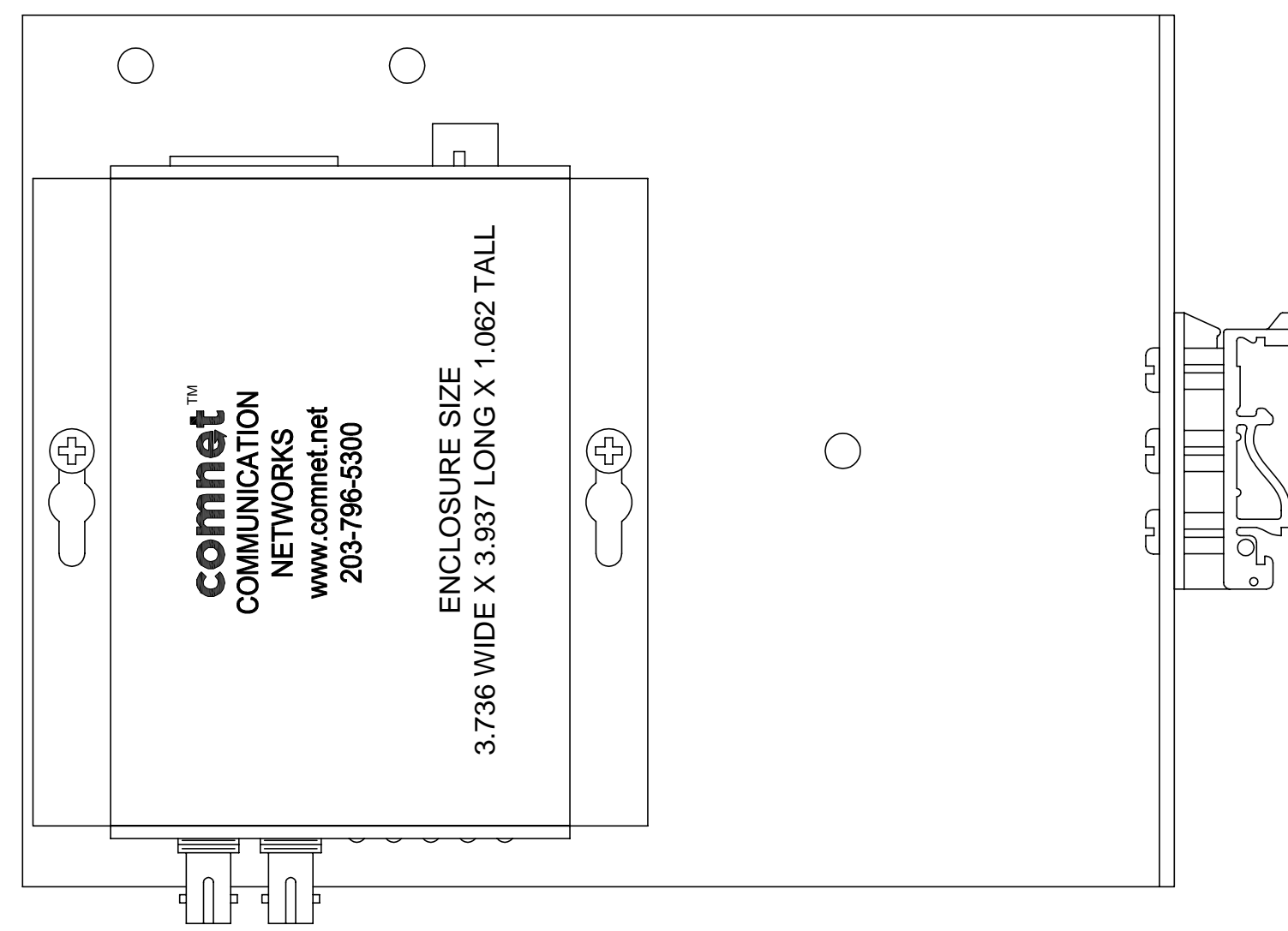
ENCLOSURES IN VERTICAL POSITION USE HOLES CODED "F" AND "G"
