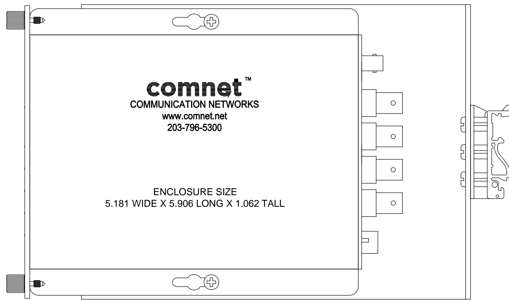
ENCLOSURE IN HORIZONTAL POSITION USE HOLES CODED "B" AND "R"
