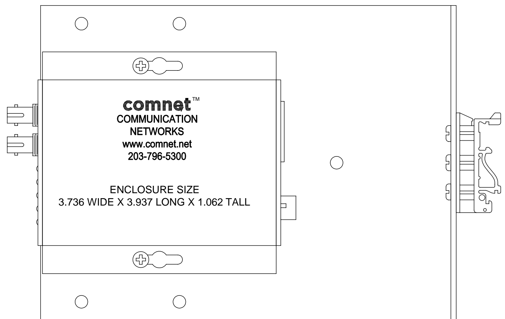
ENCLOSURES IN HORIZONTAL POSITION USE HOLES CODED "C" AND "N"
