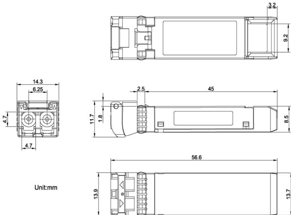
Figure 5. Outline Drawing
